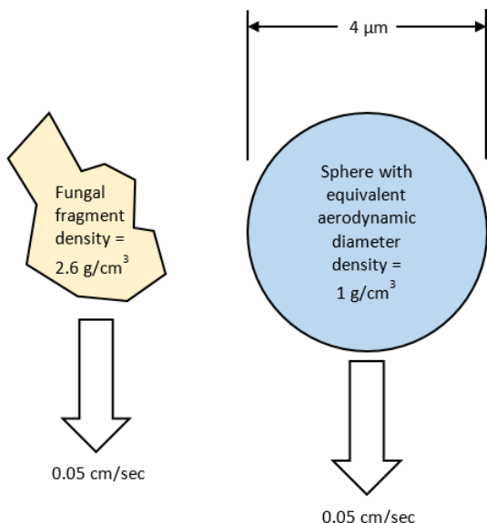
Figure 2: Aerodynamic diameter of an aerosol particle. In this case, the fungal fragment on the left is said to have an aerodynamic diameter of 4 \mu\text{m} , since it falls at the same terminal settling velocity as a 4 \mu\text{m} sphere with a unit density.
